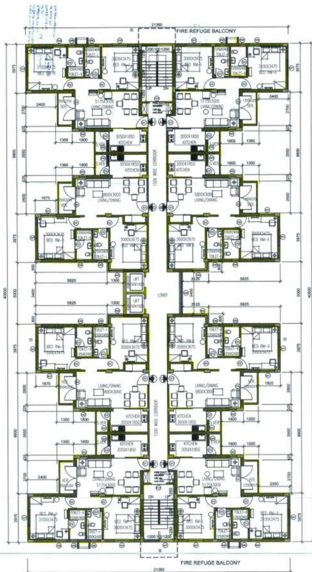
SANCTIONED TYPICAL FLOOR PLAN OF BLOCK - I & II AND COMPLETION PLAN OF BLOCK - I (STRUCTURAL PART ONLY)
