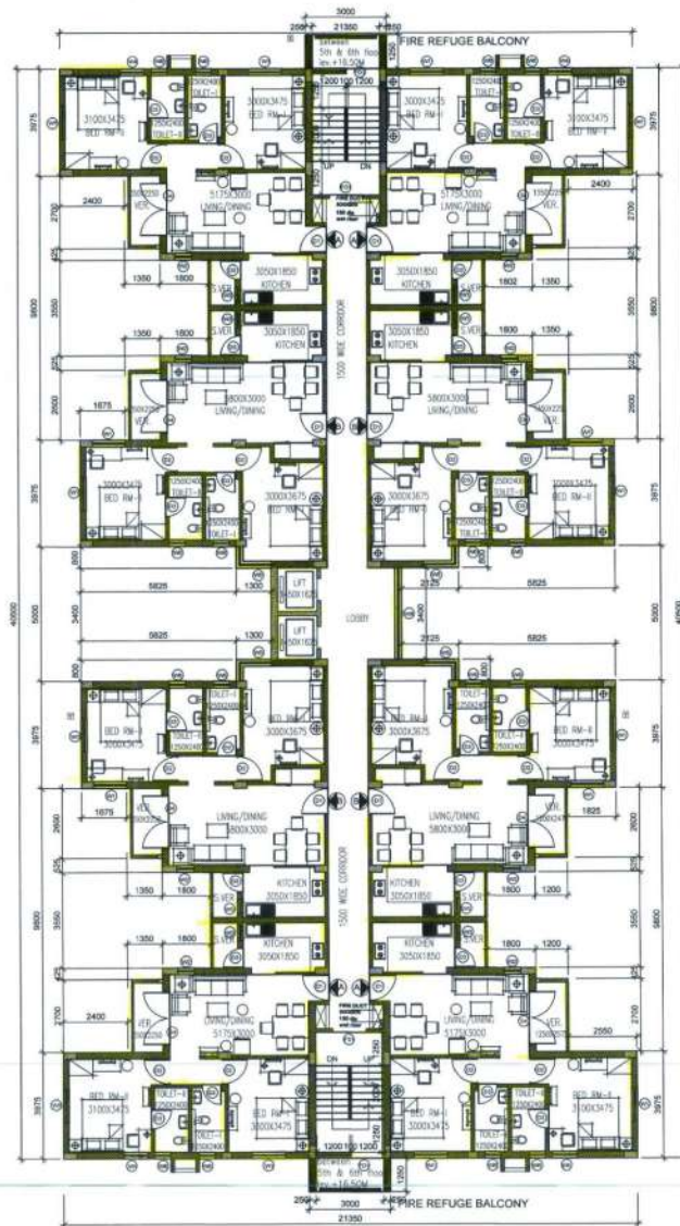
SANCTIONED PLAN 5TH & 8TH FLOOR OF BLOCK - I & II AND COMPLETION PLAN OF 5TH & 8TH FLOOR OF BLOCK - I (STRUCTURAL PART ONLY)
